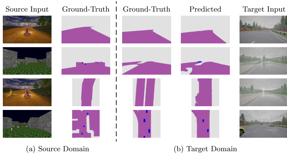
Fig. 3: We compare visual domains by their raw monocular images and corresponding semantic representations. While the domains vary significantly in their raw images, they are quite similar in their semantic modalities. However, note that the predicted modalities used by a modular pipeline are not perfect. For example, in the bottom-most row, the map-view prediction fails to capture the yellow car in view directly left of the agent. When supplied to the downstream driving policy, this vision failure can result in unintended behavior.
